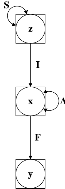
Figure D.3 Structural equation model for y variables
